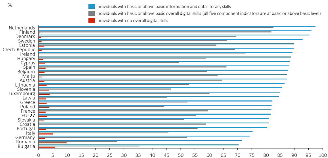
FIGURE 3 Digital skills
